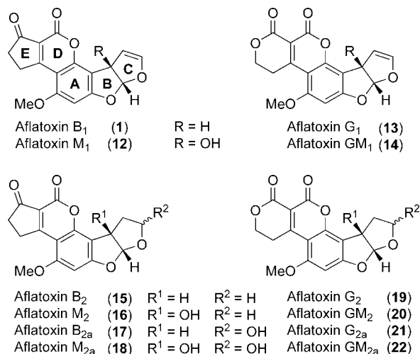
Figure 2. Aflatoxins.
