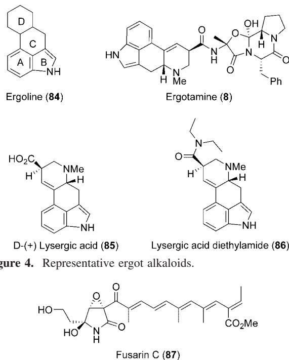
Figure 5. Fusarin C ( 87 ).
