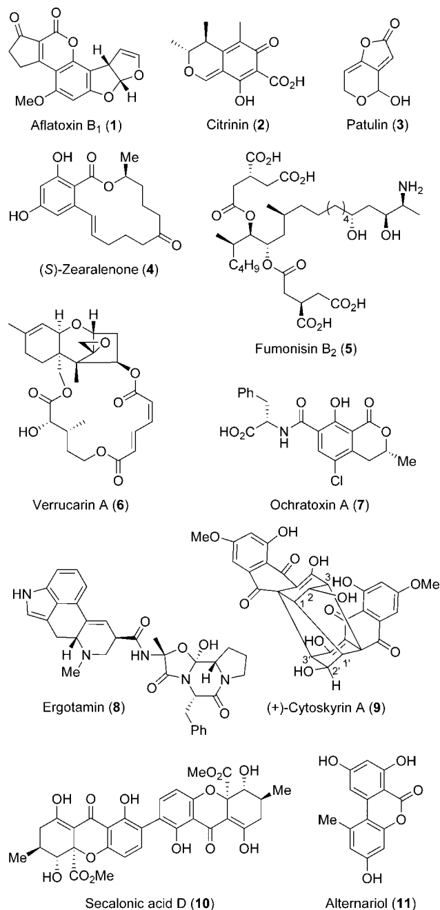
Figure 1. Important mycotoxins.
